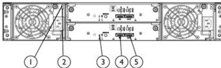
MSA 2040 LFF Disk Enclosure Rear Panel components
