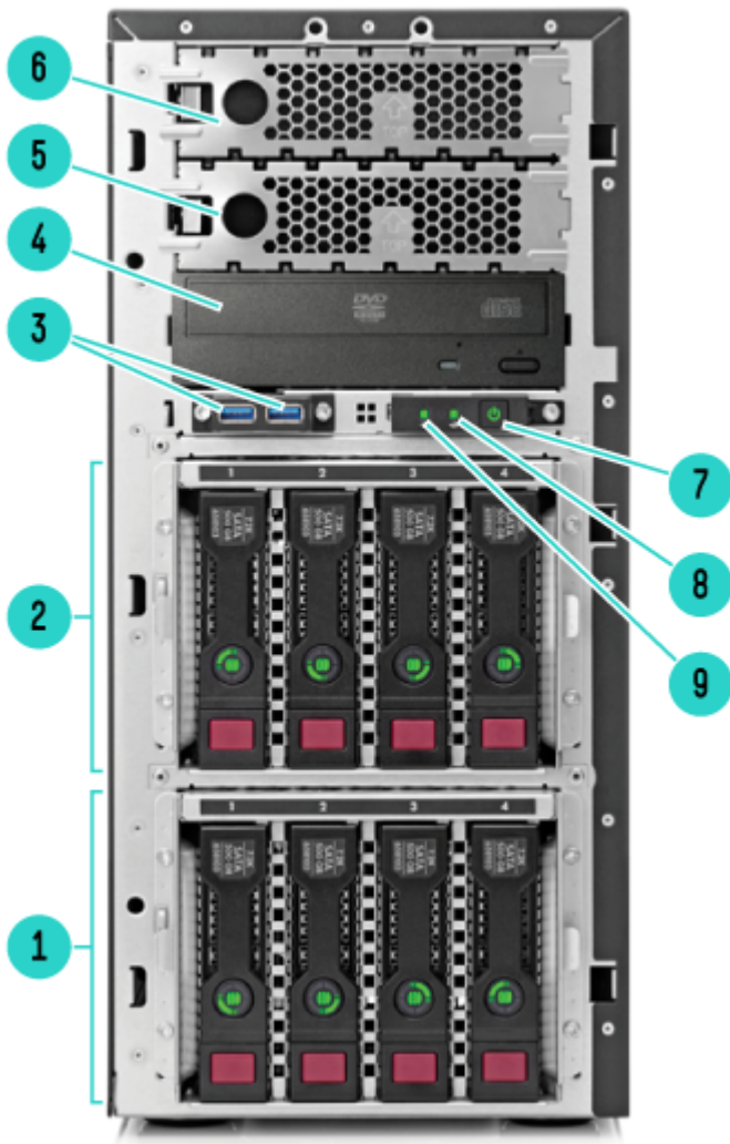
Front View details for Tower (LFF)
